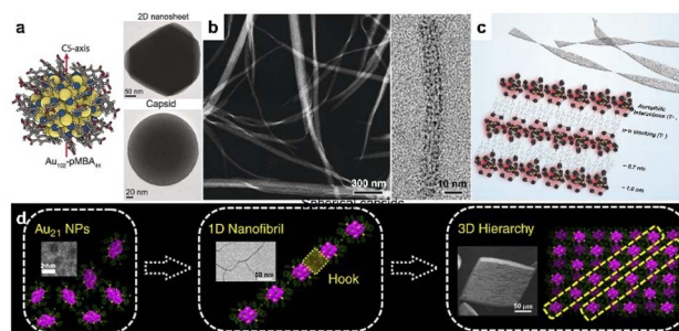
Fig. 1 Noble cluster assemblies. (a) Colloidal crystallization of \text{Au}_{102}\text{-}p\text{MBA}_{44} clusters into 2D nanosheets and spherical capsids. Reproduced from ref. 37 . (b) HRTEM images of nanoribbons. (c) Schematic illustration of self-assembly of \text{Au}_{25}(p\text{-MBA})_{18}^- into nanoribbons. Reproduced from ref. 38 . (d) The hierarchical fibrous (1D to 3D) assembly of \text{Au}_{21} clusters. Reproduced from ref. 39 .
