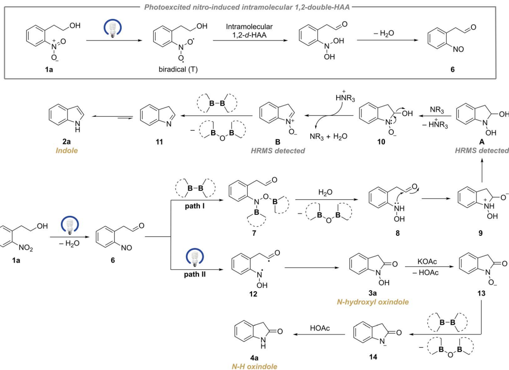
Scheme 7 Proposed mechanisms for the generation of indoles, N–OH oxindoles and N–H oxindoles.
