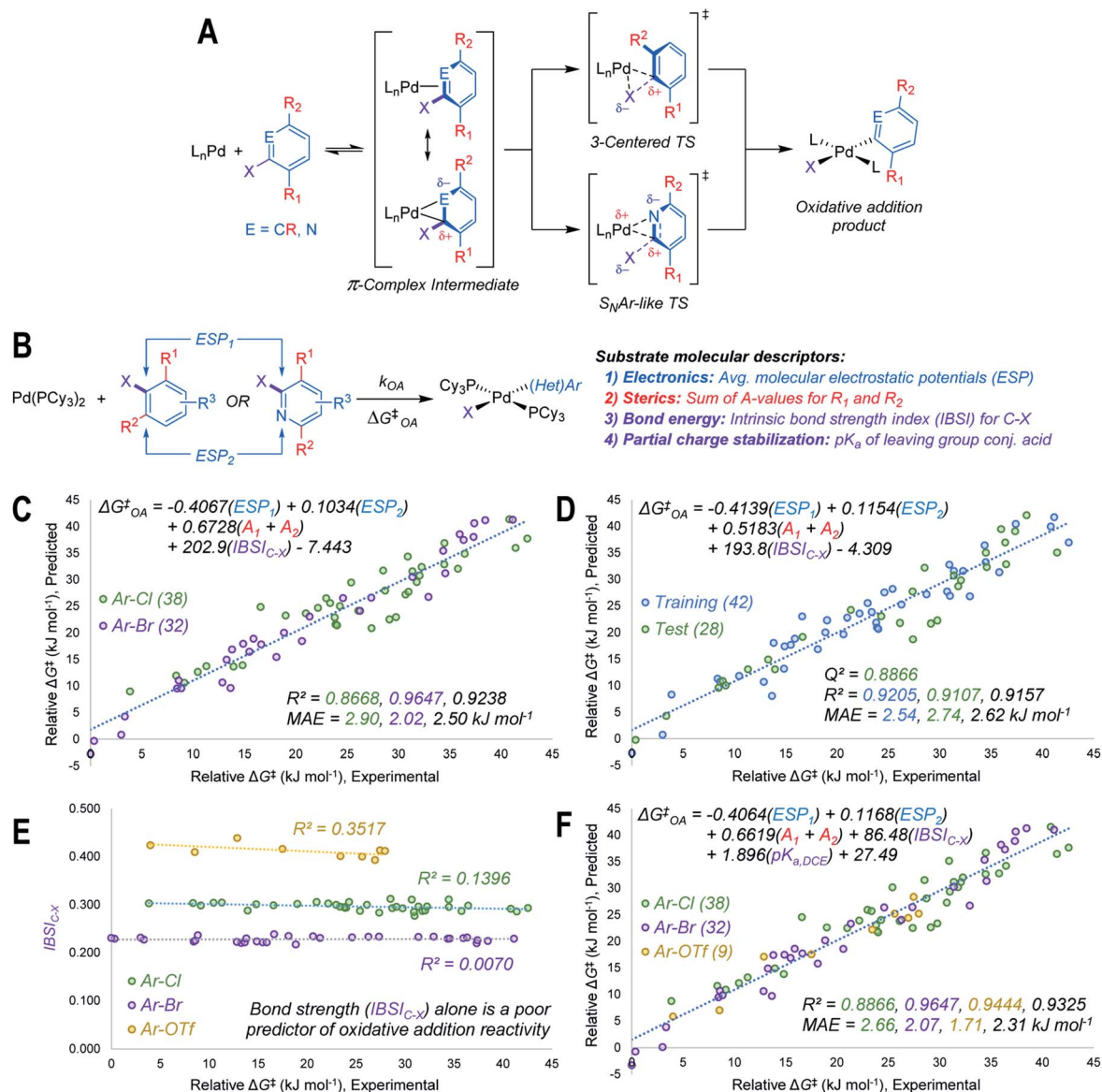
Fig. 2 Design and performance of a quantitative reactivity model for oxidative addition to Pd(0). (A) General mechanism for oxidative addition to L n Pd(0), with π-complex intermediate preceding either Pd insertion into C–X bond, or an S N Ar-like displacement of X. (B) Molecular descriptors used to model oxidative addition reactivity as a function of substrate structure. (C) Multivariate linear regression model of ΔG OA ‡ for 70 Ar–Cl and Ar–Br substrates in THF, including all data points in regression analysis. (D) Representative multivariate linear regression model generated using a 60/40 training/test split. (E) Univariate plot of IBSI C-X versus ΔG OA ‡ for Ar–Cl, Ar–Br, and Ar–OTf, revealing that bond strength is poorly correlated to ΔG OA ‡ within each leaving group set. (F) Unified linear regression model of ΔG OA ‡ for Ar–Cl, Ar–Br, and Ar–OTf substrates in THF, including all data points in regression analysis. MAE = mean absolute error. Colour-coding on R 2 , Q 2 , and MAE values corresponds to the matching data subset, values in black are for all data.
