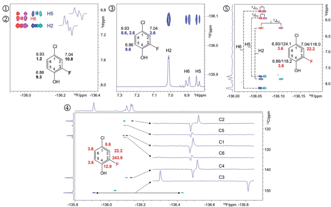
Fig. 4 Regions of the 500 MHz NMR spectra acquired with the pulse sequences presented in Fig. S8–S12† showing chemical shift correlations for compound 9. In addition to 2D cross peaks, the figures display the structure of 9 with selected NMR parameters, and where appropriate, F_2 traces showing the fine structure of cross peaks. ① Overlay of the 2D ^1\text{H} , ^{19}\text{F} HETCOR (blue/turquoise) and ② 2D ^1\text{H} , ^{19}\text{F} TOCSY-HETCOR (red/magenta) cross peaks. The TOCSY spectrum was left-shifted to facilitate identification of signals. F_2 traces through H2 and H5 cross peaks from the HETCOR spectrum are shown. ^1\text{H} chemical shifts and J_{\text{HF}} values (bold) are displayed on the structure; ③ A 2D ^{19}\text{F} , ^1\text{H} CP-DIPS13-DIPS12 spectrum; F_2 trace at the ^{19}\text{F} chemical shift of 9 is shown; ^1\text{H} chemical shifts and J_{\text{HH}} values (blue) are displayed on the structure; ④ A 2D ^{19}\text{F} , ^{13}\text{C} HMBC spectrum optimised for ^nJ_{\text{FC}} coupling constants. Internal F_1 and F_2 projections and F_2 traces at the ^{13}\text{C} chemical shifts of 9 are displayed; the J_{\text{FC}} values are shown in red; ⑤ overlay of two edited 2D(3,2) ^1\text{H}^{13}\text{C} correlation spectra containing individual cross peaks of the F_1 doublets that code for ^{13}\text{C} chemical shifts. Blue/turquoise and red/magenta colours indicate antiphase J_{\text{FC}} F_2 doublets in each spectrum. The internal F_1 projection of one of the spectra is displayed. Vertical lines connect the corresponding signals with their midpoint marking the ^1\text{H} chemical shifts. The ^1\text{H}/^{13}\text{C} chemical shifts and J_{\text{FC}} coupling constants (red) are indicated. These active coupling constants appear in antiphase, which can cause partial signal cancellation. Thus, to obtain more accurate values it is best to determine them from a ^1\text{H} coupled ^{19}\text{F} spectrum. The H6,F cross peak only appears in the 2D ^1\text{H} , ^{19}\text{F} TOCSY-HETCOR spectrum (②, Fig. 4) because the J_{\text{H6,F}} coupling constant is too small to generate a response in the former experiment. A 2D ^{19}\text{F} , ^1\text{H} CP-DIPS13-DIPS12 (③, Fig. 4) serves to extend the proton networks beyond the protons coupled to ^{19}\text{F} , similarly to 2D ^1\text{H} , ^{19}\text{F} TOCSY-HETCOR experiment. However, as a ^1\text{H} -detected experiment, it provides values of J_{\text{HH}} coupling constants that are beneficial to the structure determination process. A 2D ^{19}\text{F} , ^{13}\text{C} HMBC spectrum optimised for ^nJ_{\text{FC}} coupling constants (④, Fig. 4) provides the chemical shifts and ^nJ_{\text{FC}} coupling constants of all ^{19}\text{F} -coupled carbons. For one-bond ^{19}\text{F} - ^{13}\text{C} correlations, the sensitivity of the experiment can be enhanced by optimising the polarisation transfer periods for ^1J_{\text{FC}} coupling constants (pulse sequence of Fig. S11†). If the values of ^1J_{\text{FC}} coupling are known, the HMBC experiment can be set up to yield the one-bond correlations as well. Finally, the outcome of a simultaneous ^1\text{H}^{13}\text{C} correlation is illustrated in ⑤ (Fig. 4). This intrinsically 3D experiment has been modified using the principles of reduced dimensionality 83,84 to produce a (3, 2)D experiment. Here, the ^{13}\text{C} chemical shift is coded in the ^1\text{H} dimension by the width of the F_1 -doublet. In this experiment two interleaved spectra are acquired, which contain in-phase or antiphase F_1 doublets. Editing of these spectra increases the S/N ratio and removes half of the cross peaks in each spectrum, thus reducing spectral overlap.
