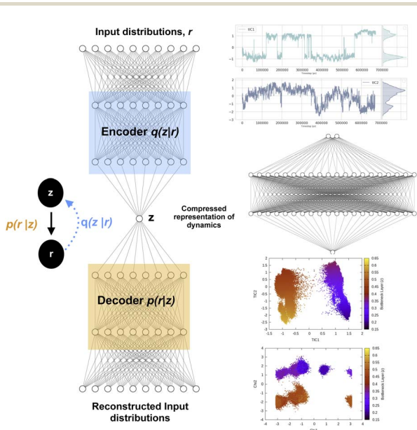
Fig. 12 Left panel showing a typical architecture of deep neural network based variational autoencoder. The input distributions r can be probability distributions of geometric variables, TICs, DMD etc. Right panel shows how latent layer of variational autoencoder learned the dynamics of the system using TICs as inputs. TICs were generated using \chi_1 and \chi_2 angles of residues present in the flap region of plasmeppsin-II (Table 1 in ESI†) with lag-time 1000. Following hyperparameters were used during the training process of VAE, no of hidden layers = 2, no of neurons in each hidden layer = 20, epochs = 100, batch size = 500, learning rate = 1e - 2 .
