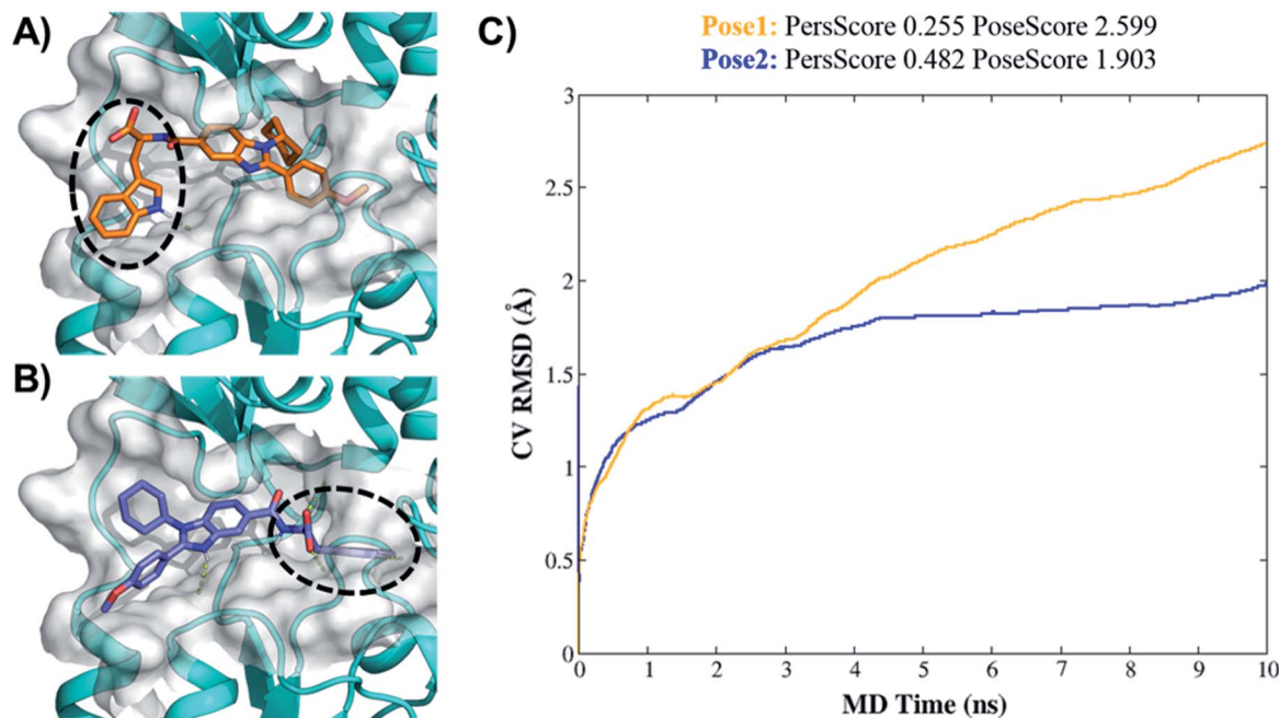
Fig. 4 Binding pose metadynamics to identify the most stable orientation. (A) Pose1 of 7d (initial pose). (B) Pose2 of 7d (IFD-pose). (C) The average RMSD of 7d during the 10 \times 10 ns metadynamics runs in pose1 (orange line) and pose2 (blue line).
