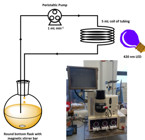
Fig. 6 Schematic representation of the continuous reaction set up used to reduce the time required for the Minisci-type reaction. Inset picture shows the Easy-Photochem flow system from Vapourtec equipped with the UV-150 photoreactor.
