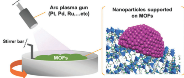
Fig. 3 Schematic illustration of the preparation of M/MOFs through the arc plasma deposition method.
