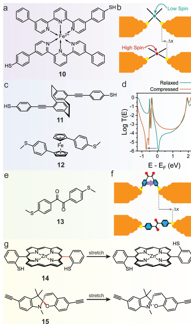
Fig. 6 Mechanically-induced changes in the molecular backbone. (a) Structure of the spin-crossover Fe(II) complex 10 and (b) mechanism of its mechanoresistive behaviour. (c) Structures of the quantum interference based mechanoinsensitive compounds discussed in this review. (d) T(E) curves for 12 , in the relaxed and compressed state. The QI feature is moved at energies below that of the LUMO in the compressed configuration, effectively lifting conductance suppression at E_F . (e) Structure of the conformationally-flexible benzil analogue discussed in the text and (f) model for its mechanoresistive behaviour. In the compressed structure the two phenyl rings rotate to a cofacial arrangement, allowing efficient through-space transport. (g) Structures for the mechanochemical switches discussed in the text. The mechanoinsensitive bond in the structure is highlighted in red. T(E) curves in (d) digitised from Camarasa-Gómez et al. 86 and replotted.
