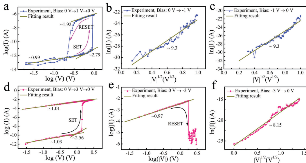
Fig. 5 Conduction mechanisms of the volatile TS and non-volatile MS in the Ag/CIS/Mo device. (a) \log(I)-\log(V) curve, the voltage swept from 0 V \rightarrow 1 V \rightarrow 0 V. (b) \ln(|I|)-|V|^{1/2} curve, the voltage swept from 0 V \rightarrow -1 V. (c) \ln(|I|)-|V|^{1/2} curve, the voltage swept from -1 V \rightarrow 0 V. (d) \log(I)-\log(V) curve, the voltage swept from 0 V \rightarrow 3 V \rightarrow 0 V. (e) \ln(|I|)-|V|^{1/2} , the voltage swept from 0 V \rightarrow -3 V. (f) \ln(|I|)-|V|^{1/2} , the voltage swept from -3 V \rightarrow 0 V.
