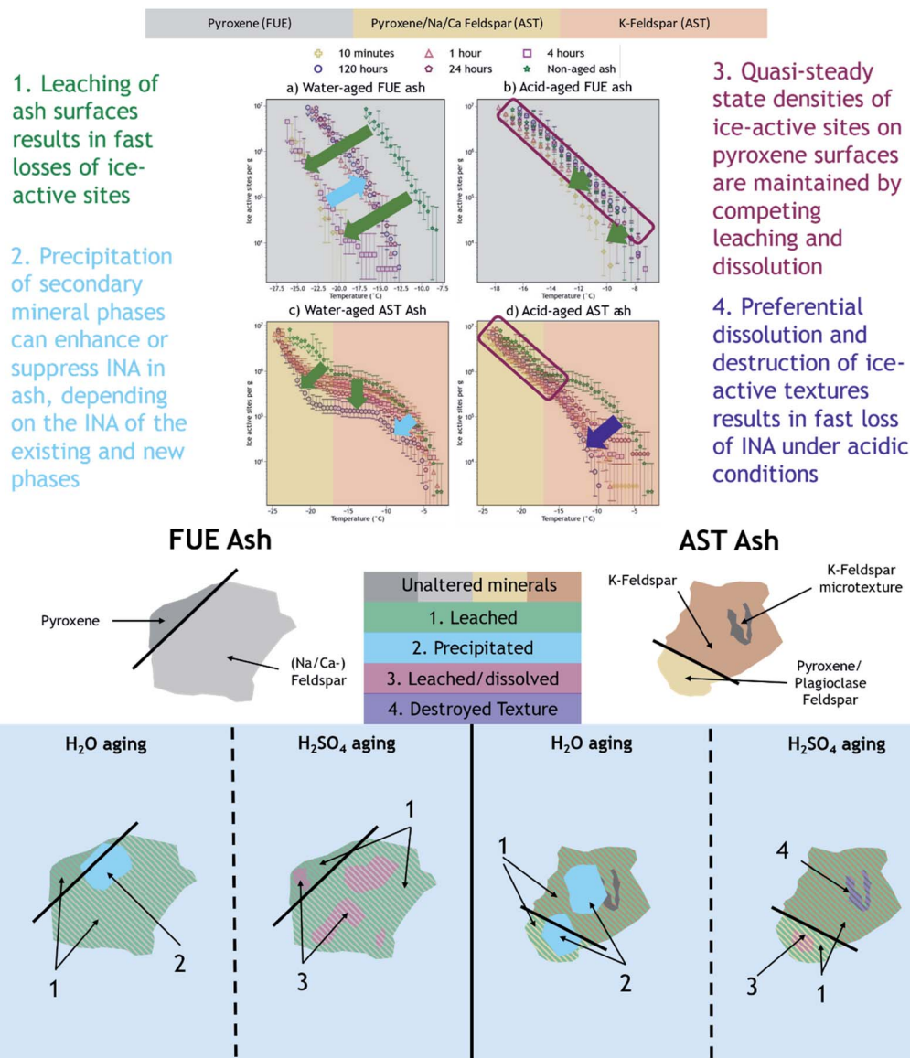
Fig. 4 Attribution of ice nucleation spectral features to specific mineral phases and summary of proposed mechanisms by which chemical aging impacts the INA of FUE and AST ash. Note the full composition of each ash is not represented because not all minerals are expected to contribute to the observed ash INA.
