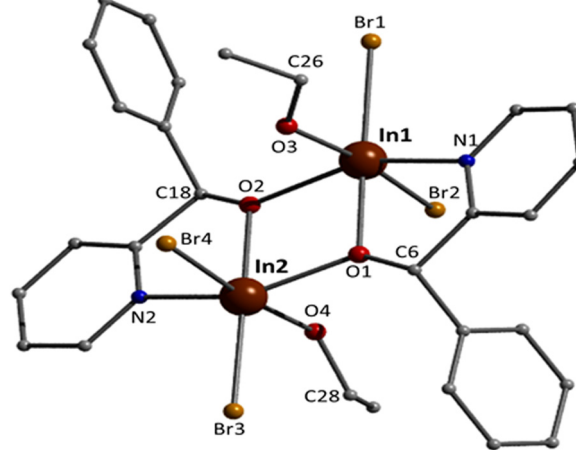
Fig. 3 Partially labelled plot of the structure of the molecule [In 2 Br 4 {(py)(ph)CH(O)} 2 (EtOH) 2 ] that is present in complex 4. H atoms are omitted for clarity. Colour code: C, grey; N, blue; O, red; Br, orange; In, brown.
