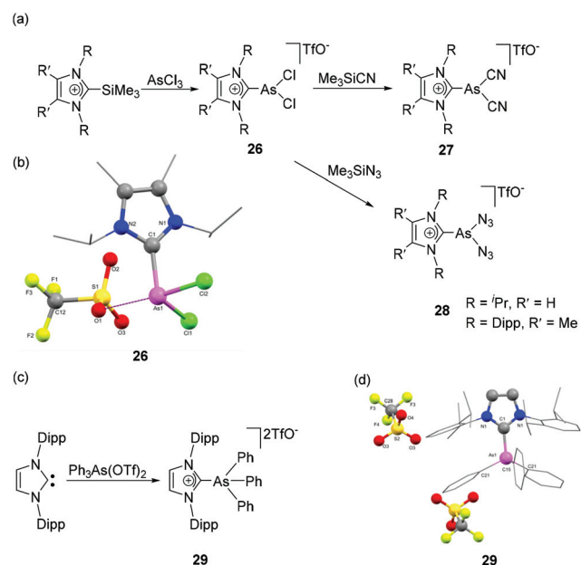
Fig. 10 Syntheses of NHC-stabilized cationic arsenic species 26–29 (a) and (c); solid-state structures of 26 (b) and 29 (d).
