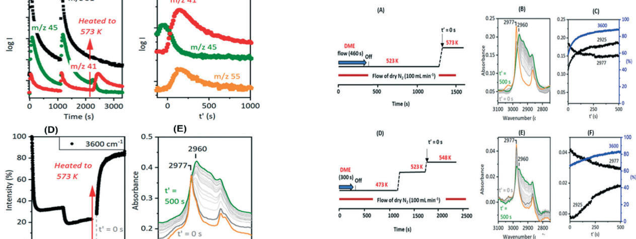
Fig. 10 T-jump experiments with DME. (A) Schematic of experiment in which a SAPO-34 crystal was exposed to DME at 523 K then the temperature ramped to 573 K. (B) Expansion of difference spectra in the \nu(\text{CH}) region shows spectrum immediately prior to T-jump (orange trace) then changes occurring following T-jump (spectra shown at 20 s intervals). (C) Band absorbance at 2925 and 2977 \text{cm}^{-1} versus time following T-jump, and \nu(\text{OH}) intensity relative to dehydrated crystal. (D) Schematic of experiment in which a SAPO-34 crystal was exposed to DME at 473 K then the temperature ramped first to 523 K then to 548 K. (E) Expansion of \nu(\text{CH}) region shows spectra immediately prior to T-jump from 523 K to 548 K (orange trace) then changes occurring following T-jump to 548 K (spectra shown at 20 s intervals). (F) Band absorbance at 2925 and 2977 \text{cm}^{-1} versus time following T-jump to 548 K, and \nu(\text{OH}) intensity relative to dehydrated crystal.
