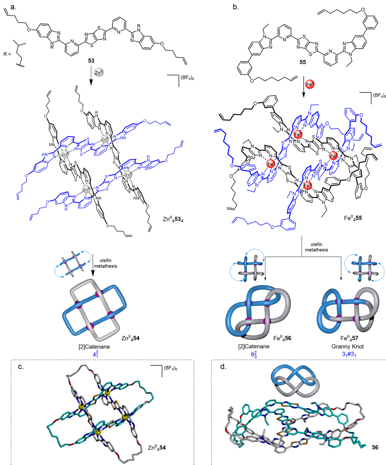
Fig. 20 Synthesis of 2 × 2 interwoven molecular grids and their closures by olefin metathesis to generate (a) Solomon link 54 , 14 or (b) 6_{\text{F}3} link 56 and granny knot 57 , 15 X-ray crystal structures of (c) \text{Zn}^{\text{II}} 54 and (d) demetallated link 56 .
