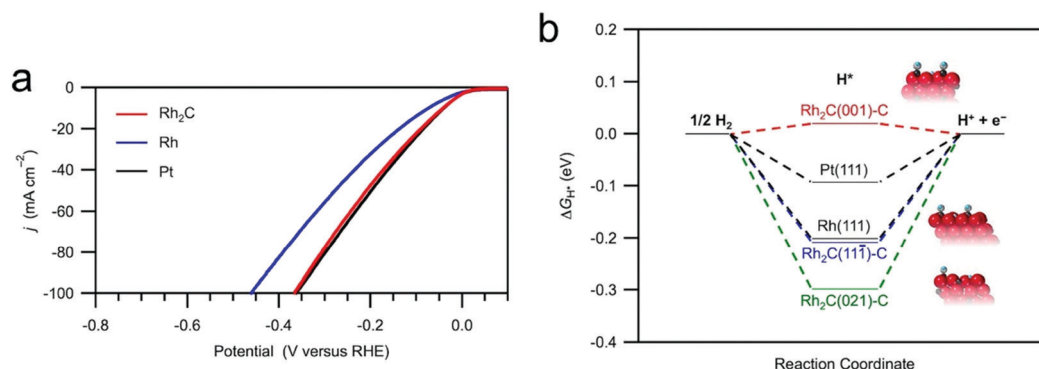
Fig. 65 (a) The HER polarisation curves of 20 wt% Rh 2 C/C (red), Pt/C (black), and Rh/C (blue). The data were recorded in a 1.0 M KOH electrolyte with a scan rate of 50 mV s -1 . (b) The 3-state free energy diagram for HER. The structural models show the OH* pre-covered surfaces used for calculations. The blue spheres are hydrogen atoms, and the gray spheres are oxygen atoms. Reproduced with permission from ref. 1003. Copyright American Chemical Society 2020.
