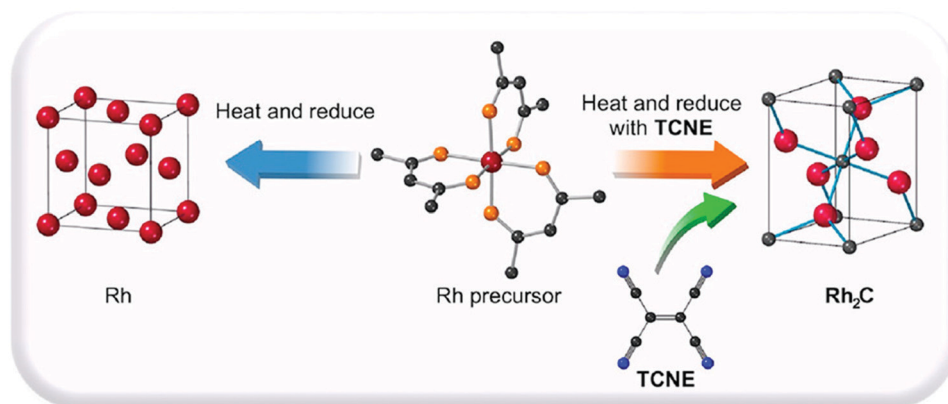
Fig. 64 Schematic presentation of the synthesis of Rh 2 C. Reproduced with permission from ref. 1003. Copyright American Chemical Society 2020.
