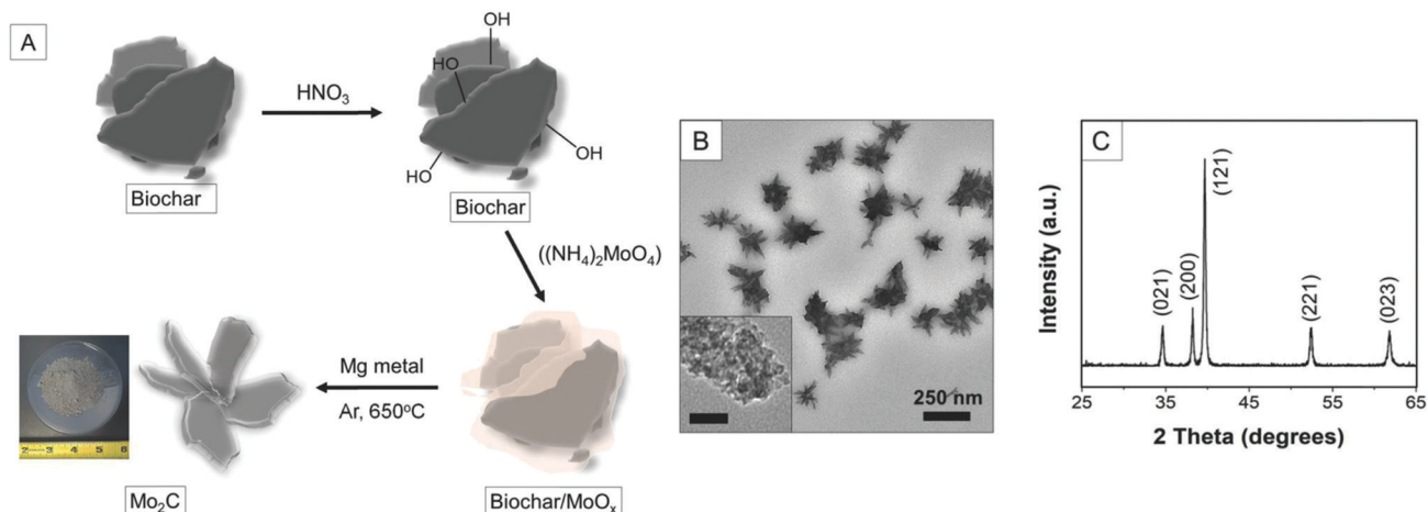
Fig. 63 (A) Schematic representation of synthesis of Mo 2 C nanostructures. (B) TEM image (inset: scale bar = 25 nm) and (C) the powder XRD pattern of Mo 2 C derived from biochar. Reproduced with permission from ref. 1002. Copyright Wiley 2018.
