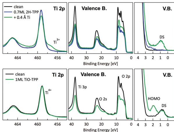
Fig. 9 Upper panels: photoemission spectra of the Ti 2p, valence band and VB zoom-in close to the Fermi level (DS) for a layer of 2H-TTPP metalated by RT deposition of 0.4 Å of Ti atoms. Lower panels: same photoemission spectra after RT deposition of 1 ML of TiO-TPP. Each molecular layer is compared with the corresponding pristine r -TiO 2 (110) surface. The Ti 2p spectra of the clean surface are renormalized to the intensity after TPP deposition; the Ti 2p spectrum after Ti deposition is shown without further renormalization to highlight the Ti tail increase. The VB spectra are simply normalized to the flux in order to highlight the change in intensity of the DS peak.
