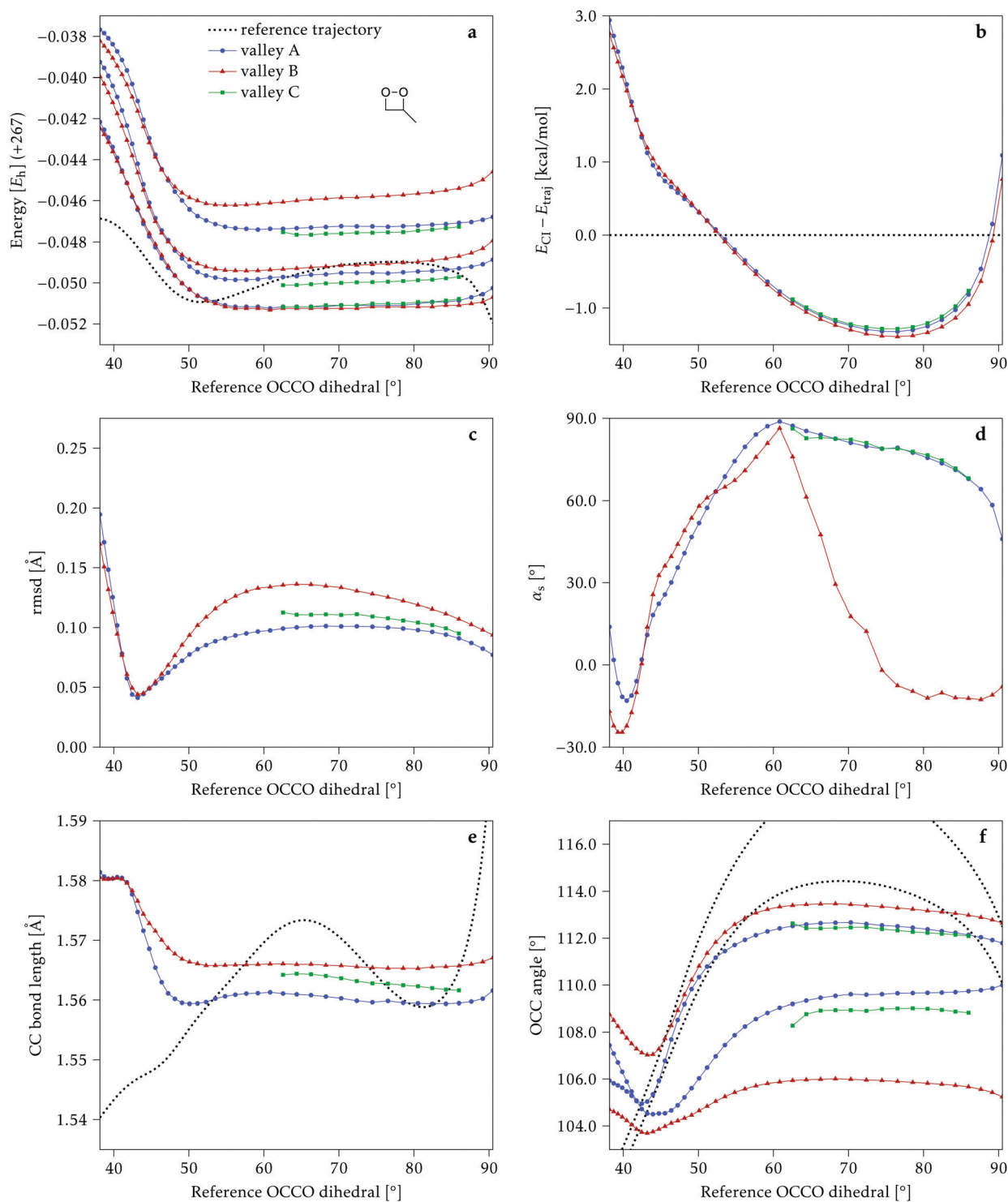
Fig. 10 Some energetic and geometric parameters along the CI valleys found for 1Me . (a) Energies of the four lowest singlet states, the first two being degenerate. (b) Energy difference between the CI and the reference trajectory. (c) Rmsd between the CI and the reference trajectory. (d) \alpha_s angle. (e) Central C–C bond length. (f) Central O–C–C angles. The values for the reference trajectory are shown as a dotted line in panels (a, b, e and f).
