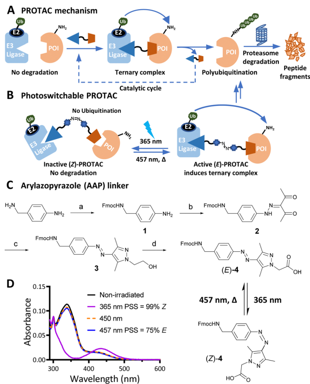
Fig. 1 (A) PROTAC-mediated protein degradation mechanism. (B) Photoswitchable PROTACs allow control of targeted protein degradation; in the example shown the active E isomer induces ternary complex formation and protein degradation, until irradiated with 365 nm light to switch to the inactive Z isomer, which fails to form an effective ternary complex. (C) Synthetic route to arylazopyrazole (AAP) photoswitchable linker 4 . Reagents and conditions: (a) Fmoc-OSu, DIPEA, DCM, RT, 16 h; 82%; (b) i. NaNO 2 , acetic acid, 37% HCl, 0 °C, 1 h; ii. acetylacetone, ethanol, sodium acetate, 0 °C to RT, 3 h; 83% over two steps; (c) 2-Hydrazinoethanol, DCM, MeOH, 50 °C, 2 h; 98%; (d) i. Dess–Martin periodinane, DMSO, RT, 16 h; ii. NaClO 2 , NaHPO 4 , 2-methylbut-2-ene, RT, 16 h; 40% over two steps. (D) Ultraviolet-Visible (UV-Vis) spectra of a 20 μM solution of 4 in water with 0.2% DMSO under the stated irradiation conditions.
