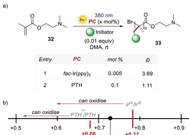
Scheme 18 (a) Polymerisation of dimethylaminoethyl methyl methacrylate. Comparison between the performances of PTH and fac -Ir(ppy) 3 . (b) Graphical depiction of the oxidation potentials (vs. SCE in MeCN) of 32 , PTH and fac -Ir(ppy) 3 .
