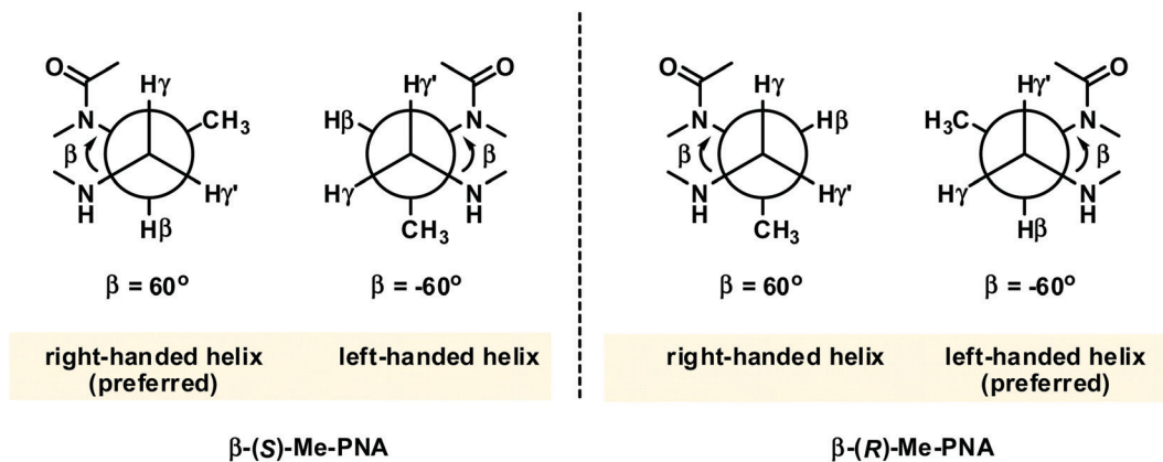
Fig. 6 The gauche conformation of the N(H)-C γ -C β -N(CO) groups necessitates pre-organization into the right-handed helix in \beta -( S )-methyl PNA. 36 The structure is viewed along the C γ -C β axis.
