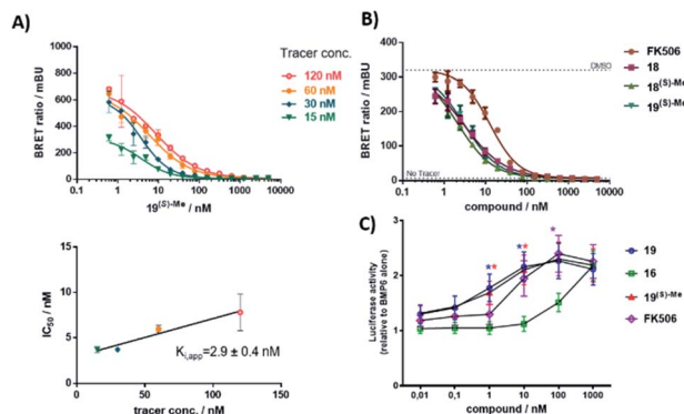
Fig. 6 (S)-Me-substituted [4.3.1] bicycles potentially block FKBP in cells. (A) Intracellular FKBP12-NLuc engagement of compound 19 (S)-Me determined by competitive NanoBRET assay. HEK293T cells stably expressing FKBP12-NLuc constructs were treated with increasing concentrations of 19 (S)-Me in the presence of varying concentrations of NanoBRET tracer as shown in the upper panel. Each curve was fitted to determine an IC 50 , which was plotted in the lower panel in dependence of the tracer concentration to determine the K_i^{app} by Cheng-Prusoff analysis. (B) Competitive NanoBRET assay for FK506 and three bicyclic compounds. NanoBRET experiments were performed in three independent cellular assays for all samples. (C) Dose responses for FK506 and three bicyclic compounds determined in an INA-6 BRE-luc reporter assay. All cells were treated with BMP-6 (7.5 ng mL -1 ) and indicated compounds for 18 hours. The measured luciferase activities were normalized to BMP-6 alone. Shown are the averages and standard error of the mean (SEM) of n = 4 biological replicates. A two-way ANOVA with Tukey's multiple comparison test and Geisser–Greenhouse correction was performed. The asterisks indicate statistical significance (* p < 0.05 ) for compound 16 vs. 19 (blue asterisks) or 19 (S)-Me (red asterisks) at 1 nM and 10 nM, and compound 16 vs. FK506 (pink asterisk) at 100 nM. The other comparisons were not significant ( p > 0.05 ).
