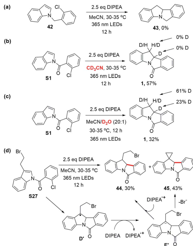
Scheme 7 Mechanistic experiments.
