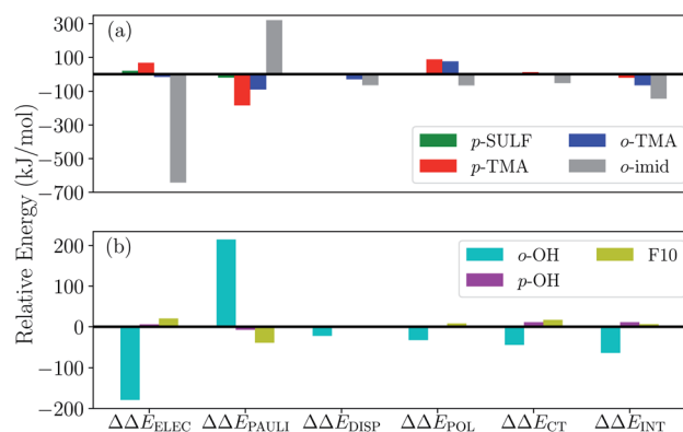
Fig. 10 Differential ALMO-EDA(sol) results (in \text{kJ mol}^{-1} ) relative to the unsubstituted [\text{FeTPP}(\text{CO}_2)]^{2-} complex: (a) results for the charged substituent groups ( -\text{NMe}_3^+ , -\text{SO}_3^- , and the methylimidazolium-carrying group); (b) results for the substituent groups that retain the net charge of the unsubstituted complex ( -\text{OH} , -\text{F} ).
