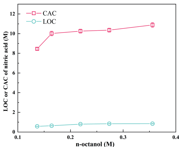
Fig. 8 LOC and CAC of nitric acid as a function of n -octanol concentration, [\text{L}^{\text{II}}] = 0.12 M.
