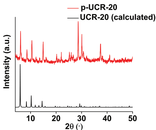
Fig. 2 PXRD patterns of UCR-20 (calculated) and p-UCR-20.
