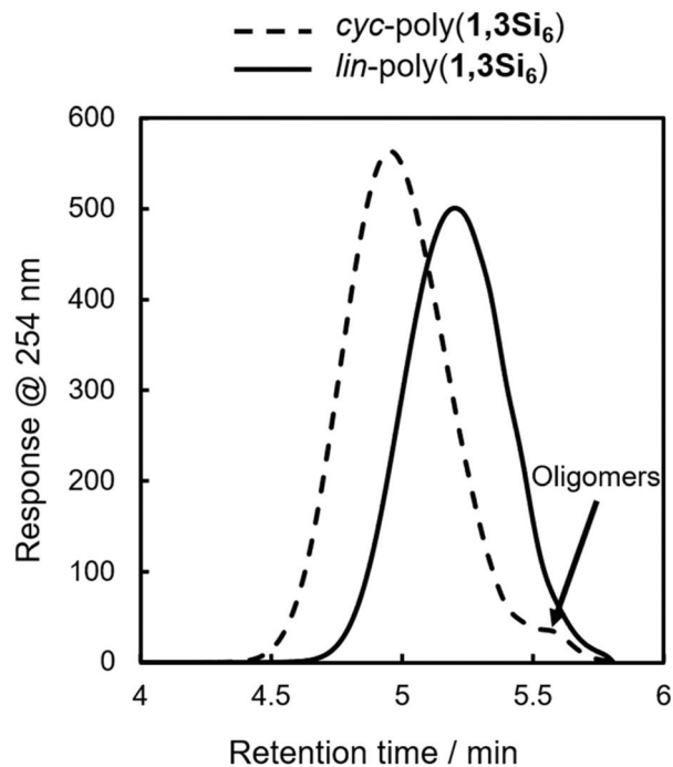
Fig. 2 GPC of cyc -poly(1,3Si 6 ) (dotted line) and lin -poly(1,3Si 6 ) (solid line). Determined relative to polystyrene standards at 254 nm (THF, [ lin -poly(1,3Si 6 )] = 1 mg mL -1 , 40 °C, 0.35 mL min -1 , 10 μL injection).
