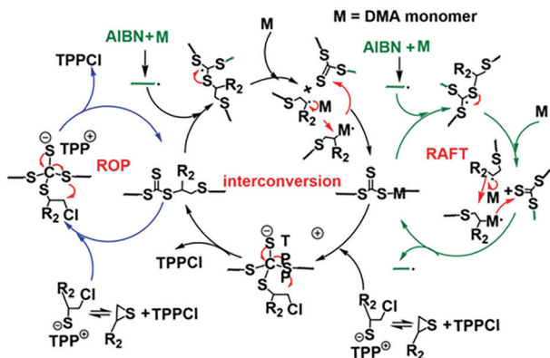
Fig. 4 Interconvertible hybrid copolymerizations of AROP and RAFT. Reproduced from ref. 23 with permission from the Royal Society of Chemistry, copyright 2019.
