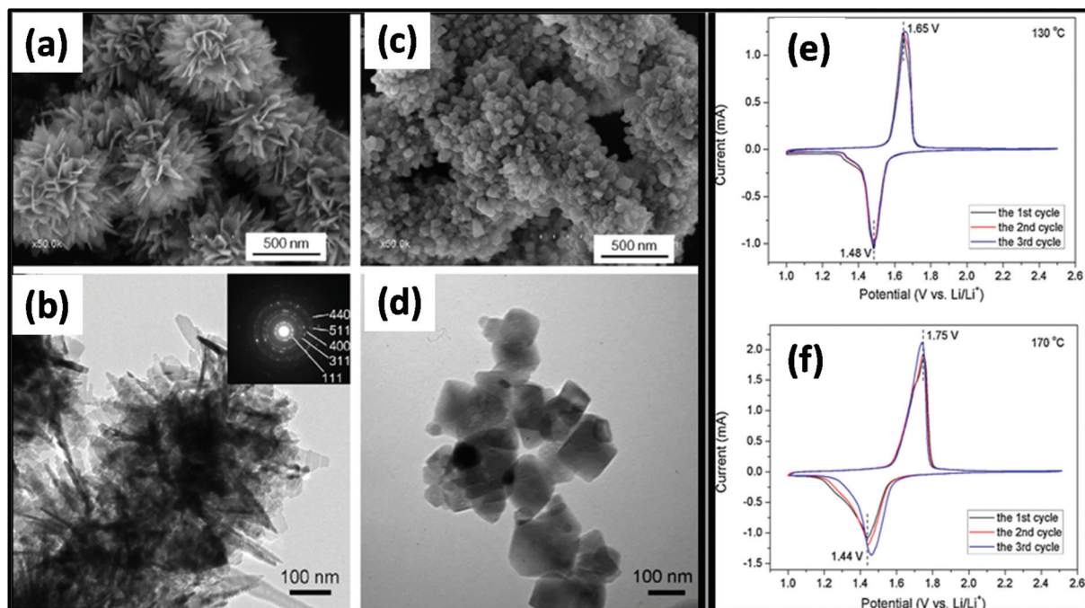
Fig. 20 (a and c) SEM images of \text{Li}_4\text{Ti}_5\text{O}_{12} synthesized at 130 \text{ }^\circ\text{C} and (b and d) TEM images of \text{Li}_4\text{Ti}_5\text{O}_{12} synthesized at 170 \text{ }^\circ\text{C} . (e and f) CV curves of \text{Li}_4\text{Ti}_5\text{O}_{12} prepared at (e) 130 \text{ }^\circ\text{C} and (f) 170 \text{ }^\circ\text{C} in the first three cycles at a scan rate of 0.2 \text{ mV s}^{-1} . Reprinted (adapted) with permission from ref. 281, copyright (2012), Elsevier B.V. All rights reserved.
