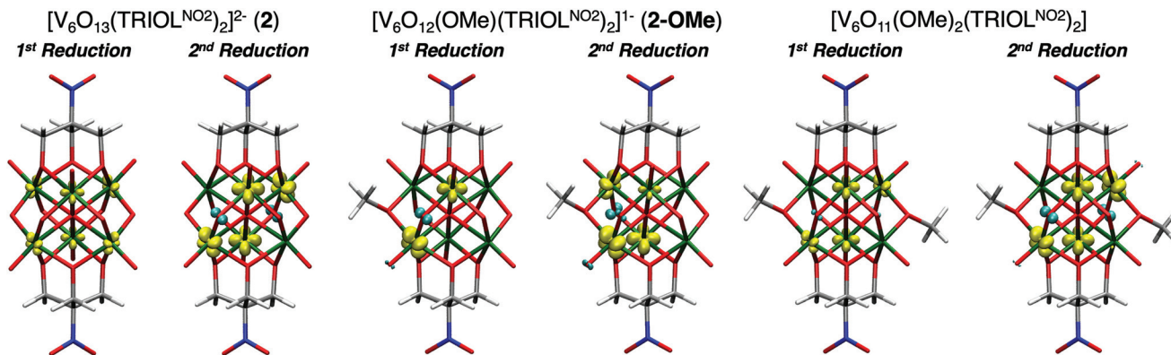
Fig. 7 Spin density of reduced 2 , 2-OMe , and para -[V 6 O 11 (OMe) 2 (TRIOL NO 2 ) 2 ] 2- at M06/def2-TZVP//M06-L/def2-TZVP,def2-SVP level of theory. Vanadium in dark green, oxygen in red, nitrogen in blue, carbon in grey, and hydrogen in white. Alpha spin density in yellow and beta spin density in cyan. Isosurface = 0.4. Additional spin density plots for reduced variants of 1-OMe and meta - 1-(OMe) 2 can be found in Fig. S17.†
