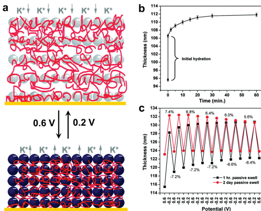
Fig. 7 (a) Schematic depiction of the reversible electrochemically-induced swelling of LBL-produced LPEI-PB NP composite films. Reduction of PB NPs causes cationic electrolyte solution to migrate into the film to maintain charge balance, resulting in significant film swelling. The opposite process happens upon PB NP oxidation. (b) Time-dependent passive swelling of LPEI-PB films in electrolyte solution as measured by ellipsometry. Film thickness sees a 17% increase from the dry state after 1 h and a 30% increase from the dry state after 2 days. (c) Electrochemically-induced active swelling of LPEI-PB films across multiple redox cycles as measured by ellipsometry. Films that were passively swollen for two days beforehand exhibited highly reversible swelling behavior, whereas those that were passively swollen for only 1 h exhibited somewhat irreversible swelling initially, eventually achieving reversibility once their thickness values converged with those of the 2-day preswollen films after repeated cycling. 169 Adapted with permission from ref. 169 (copyright 2009, American Chemical Society).
