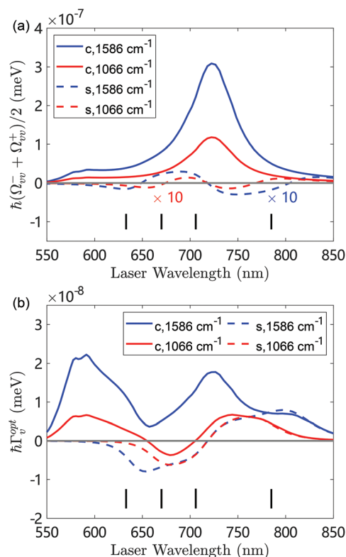
Fig. 5 (a) Vibrational frequency shift (\Omega_{\text{vw}}^+ + \Omega_{\text{vw}}^-)/2 and (b) effective optomechanical damping rate \Gamma_{\text{vw}}^{\text{opt}} = \Gamma_{\text{vw}}^- - \Gamma_{\text{vw}}^+ as a function of the laser wavelength for the 1586\text{ cm}^{-1} vibrational mode (blue lines) and the 1066\text{ cm}^{-1} vibrational mode (red lines). The solid and dashed lines are the results from the continuum-field model (labeled as "c") and the single-mode model (labeled as "s"), respectively. The vertical lines indicate wavelengths at 633 nm, 670 nm, 705.9 nm and 785 nm used for later simulations. The laser intensity is 1\ \mu\text{W}\ \mu\text{m}^{-2} and other parameters are specified in the text.
