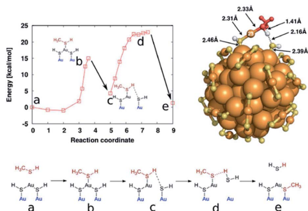
Fig. 7 Scheme of ligand exchange process with methane thiol and \text{Au}_{102}(\text{SR})_{44} clusters. Top-left panel: energy behavior during exchange process (corresponding configuration were depicted as a sketch in the bottom panel); top-right panel: hemiring-like intermediate c . Configurations close to b and d have been confirmed to be at the local energy maximum by structural relaxations to the intermediate and final states. Adapted with permission from ref. 88. Copyright 2012 American Chemical Society.
