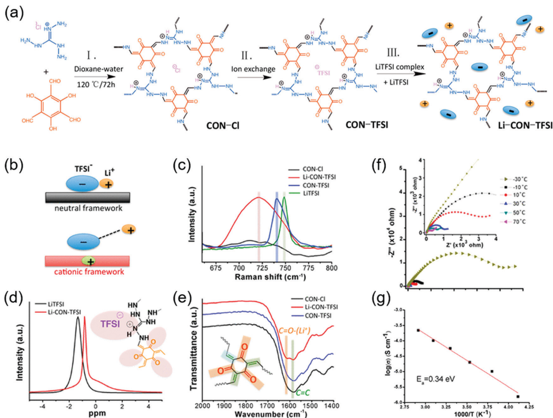
Fig. 21 Self-exfoliated, cationic COFs as Li-ion conductor. (a) Design and synthesis of cationic COFs for Li + conduction. (b) Differences in ion pair formation at neutral and cationic COF. (c) Raman spectra (d) 7 Li MAS NMR spectra (e) FTIR spectra of COFs and Li-CON-TFSI, establishing lithiation of COFs. (f) Temperature-dependent EIS of Li-CON-TFSI. (g) Calculation of activation energy ( E_a ) for Li-CON-TFSI in hydrous conditions by the methods of Arrhenius. Reproduced with permission. 154 Copyright 2018, American Chemical Society.
