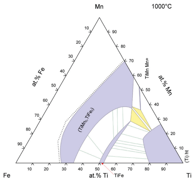
Fig. 6 Isotherm section at 1000 °C of the Ti-Fe-Mn phase diagram. Reproduced with permission from ref. 22.
