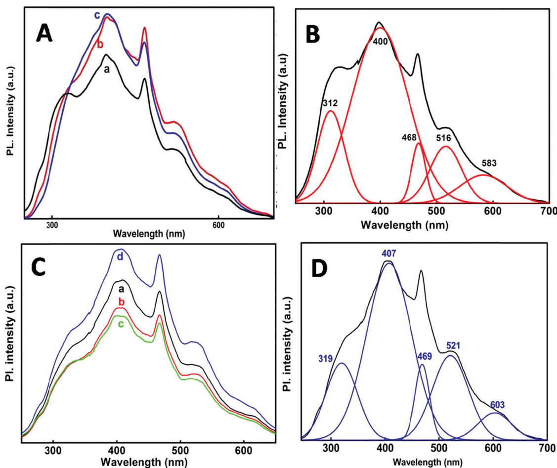
Fig. 7 (A) Room temperature PL spectra of tin oxide nanoparticles synthesized at different temperatures in reline ( \lambda_{exc} = 220 nm), (a) 50 °C; (b) 80 °C; and (c) 98 °C. (B) De-convoluted fitting plot of the PL spectrum of the nanoparticles obtained at 50 °C with \lambda_{exc} = 220 nm. (C) Room temperature PL spectra of tin oxide nanoparticles synthesized at different e-beam irradiation doses in the reline host matrix ( \lambda_{exc} = 220 nm), (a) 35 kGy; (b) 72 kGy; (c) 107 kGy and (d) 143 kGy. (D) De-convoluted fitting plot of the PL spectrum of the nanoparticles (by the e-beam irradiation method) at \lambda_{exc} = 220 nm.
