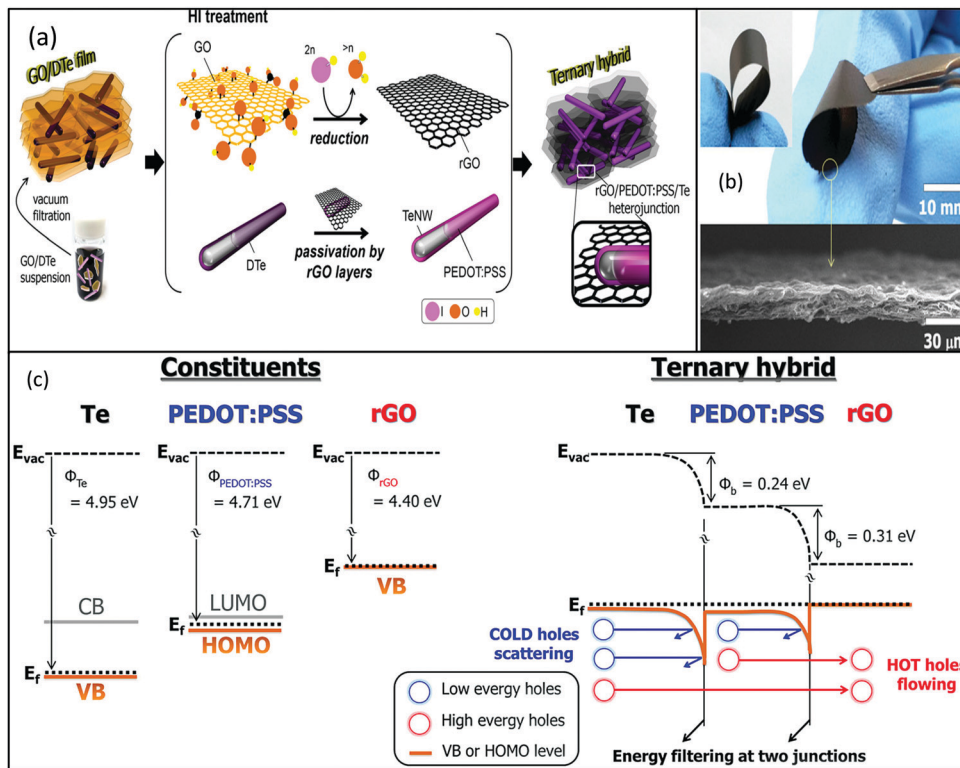
Fig. 13 (a) Synthesis of TE hybrid paper, (b) picture of prepared flexible G_{0.1}DTe_{0.9} hybrid paper, and (c) energy diagram of the rGO/PEDOT:PSS/TeNW and rGO/PEDOT:PSS of DTe. Reprinted with permission from ref. 157 (J. Choi, J. Y. Lee, S. S. Lee, C. R. Park, H. Kim, Adv. Energy Mater. 6 (2016) 1–8). Copyright (2016) John Wiley & Sons Publications.
