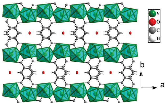
Fig. 2 The connectivity of the 2D structures through terephthalates to form a 3D structure of [\text{Y}(\text{tp})(\text{ox})_{0.5}(\text{H}_2\text{O})_2]\cdot\text{H}_2\text{O} , 1 . Note the presence of 1D water occupying the channels along the c axis. Hydrogen atoms of the water molecules are not shown.
