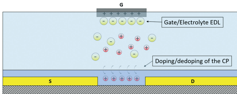
Fig. 2 The OEGFET working principle. The channel current I_D is modulated by the application of a gate voltage, which promotes the doping/dedoping of the CP layer. Since the whole volume of the CP layer is affected by the doping/dedoping mechanism, this device is characterized by a volumetric capacitance that helps to obtain high transconductances, and thus high sensitivities and low operating voltages. The doping/dedoping mechanism can be influenced by the presence of a cell layer on the surface of the CP.
