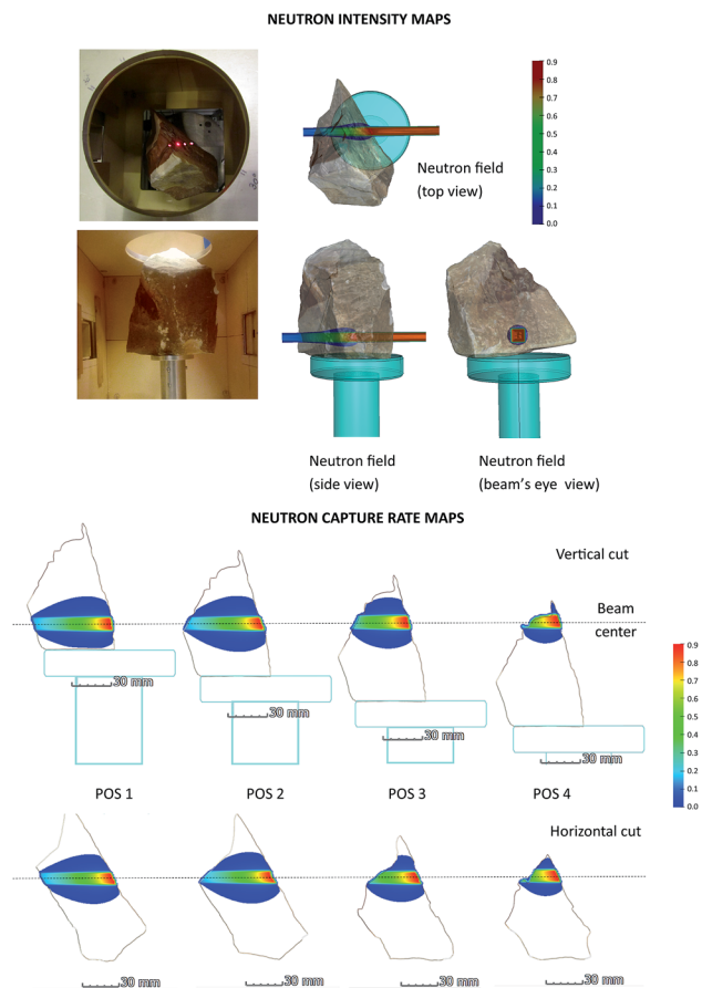
Fig. 4 A photo of the object in the sample chamber (top left), the neutron field at the bottom position of the stone object, Pos 1 (top right), and the capture reaction rate map of the ^{40}\text{Ca} isotope for all four measurement positions (bottom), indicating the local source strength of the prompt-gamma rays. Note the dark blue area around the direct beam, where only scattered neutrons are present. The experimental measurement positions are indicated in the photo by laser beam spots. Additional plots are shown in ESI 3.†
