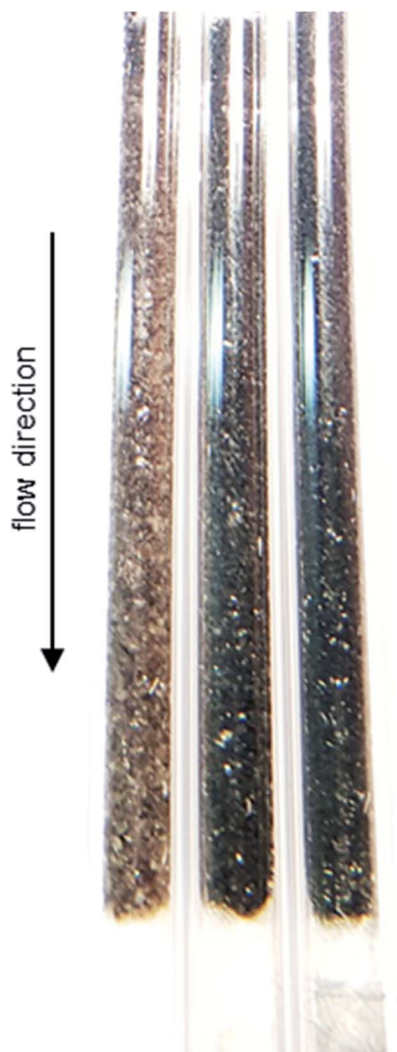
Fig. 9 Picture of the three quartz capillary reactors after PDH over GaPt/ \text{SiO}_2 SCALMS with an atomic ratio of Ga/Pt of 55 at 450 (left), 500 (middle), and 550 °C (right) visualising the temperature dependent deposition of carbonaceous species on the catalyst. It is noted, that small amounts of coke also formed on the second part of the quartz wool plug at the end of the catalyst bed after operation at 550 °C. The first part of this quartz wool plug is seemingly not affected, most likely as it is still within the isothermal zone of the fixed-bed reactor.
