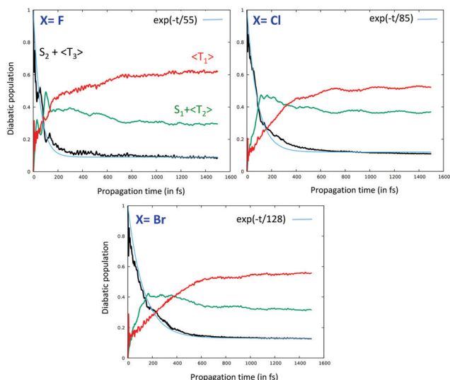
Fig. 10 Time-evolution of the population of the low-lying T_3 , S_2/T_2 and S_1/T_1 excited states in [Re(F)(CO) 3 (bpy)] (a), [Re(Cl)(CO) 3 (bpy)] (b) and [Re(Br)(CO) 3 (bpy)] (c). For the sake of clarity, the S_2/T_3 and S_1/T_2 populations are summed up. 97
