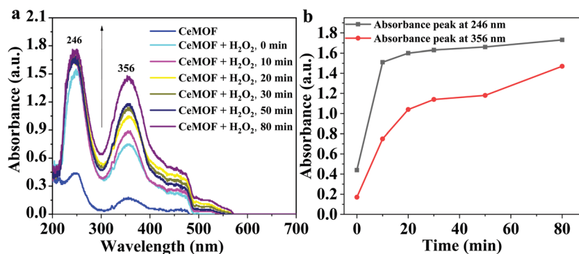
Fig. 8 (a) UV-Vis absorption spectra of Ce-MOF without and with H 2 O 2 over time, and (b) the absorbance intensities at wavelengths 246 nm and 356 nm.
