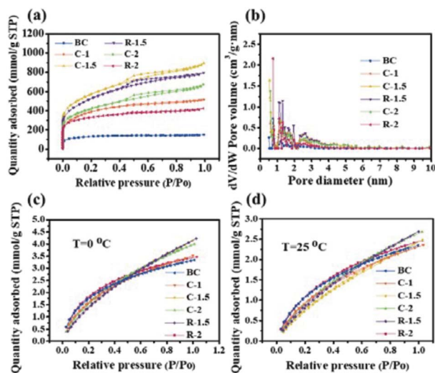
Fig. 2 N_2 adsorption–desorption isotherms (a), pore size distributions (b) and CO_2 adsorption isotherms measured at 0 (c) and 25 \text{ }^\circ\text{C} (d) of the as-prepared porous carbons.
