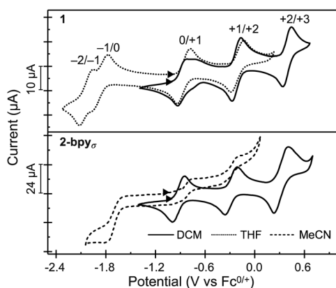
Fig. 4 Solution and solid state cyclic voltammograms of 1 and 2-bpy _{\sigma} , respectively, recorded in DCM (solid lines), THF (dotted lines) or MeCN (dashed lines) solutions of \text{TBAPF}_6 (0.1 M), at a scan rate of 200 \text{ mV s}^{-1} . The data for 2-bpy _{\sigma} was recorded by dropcasting crystalline material on a glass carbon disk electrode.
