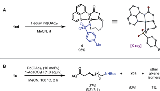
Scheme 2 Mechanistic experiments.
