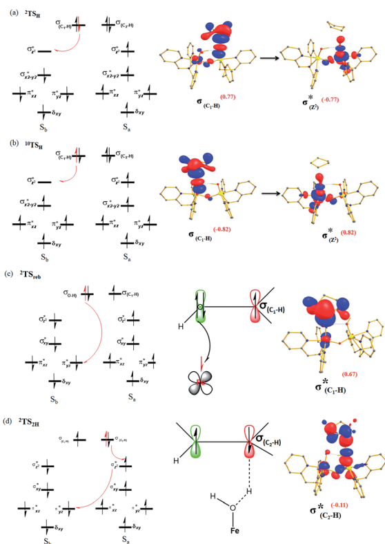
Fig. 3 Electron shift diagrams of \text{I-TS}_{\text{H}} for both (a) \text{I}^{-2}\text{TS}_{\text{Hhs-hs}} , (b) \text{I}^{-10}\text{TS}_{\text{Hhs-hs}} , (c) \text{Ia}^{-2}\text{TS}_{\text{rebhs-hs}} and (d) \text{Ib}^{-2}\text{TS}_{2\text{Hhs-hs}} with SNOs and their occupation (noted in parentheses).
