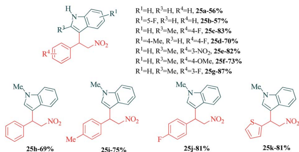
Scheme 7 Friedel-Crafts alkylation of indoles with nitroalkenes in water.
