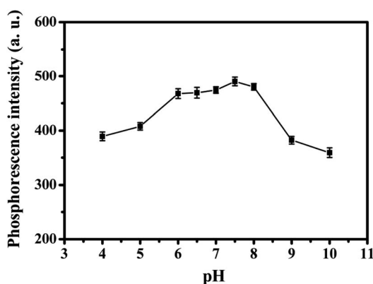
Fig. 8 Effect of pH on the RTP intensity of MPTS-ZnS QDs:Mn.
