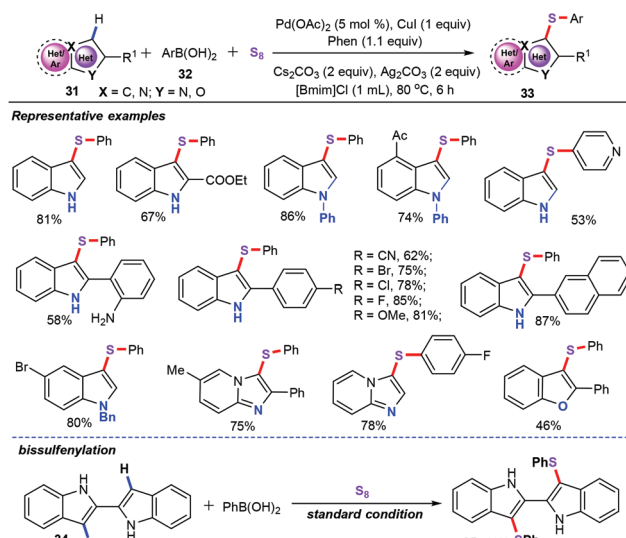
Scheme 13 Palladium-catalyzed oxidative sulfenylation of electron-rich heteroarenes.
